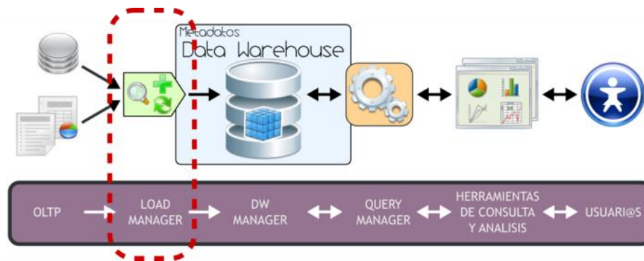
Figura 3.3: Load Manager.
