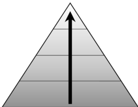
Figura 3.40: Drill-up.
