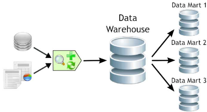
Figura 4.1: Top-Down.
