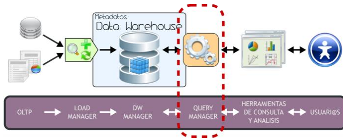
Figura 3.32: Query Manager.
