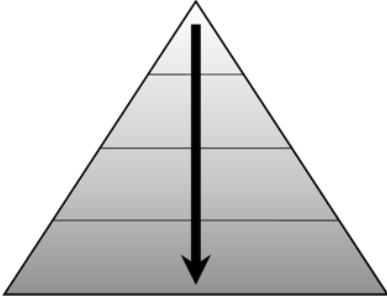
Figura 3.36: Drill-down.
