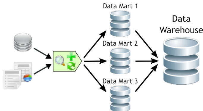
Figura 4.2: Bottom-Up
