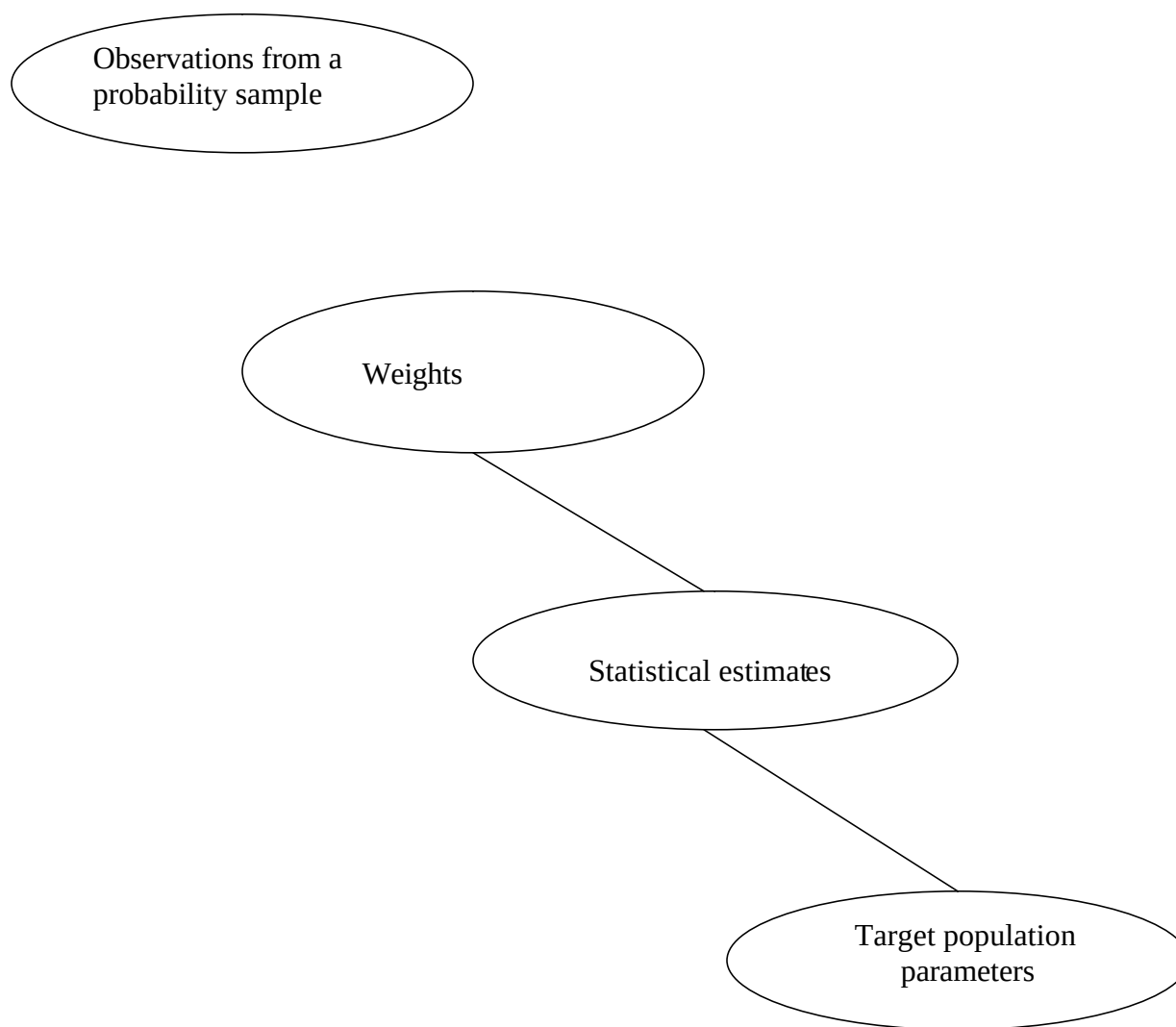
Figure 1. Application of weights and statistical estimation
